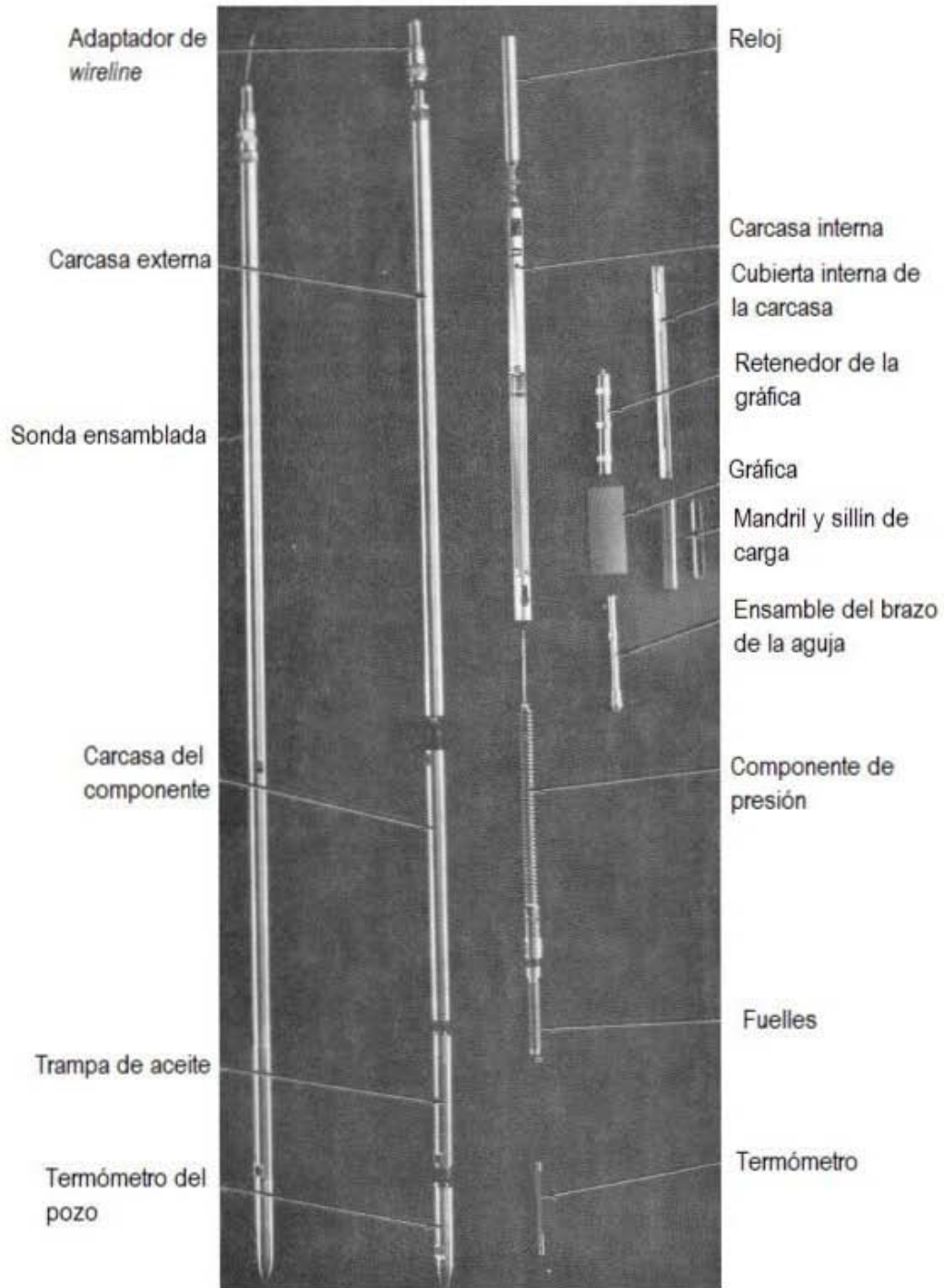
Fig. IV.2.1.1 Sonda Amereda RPG-3, (Geophysical Research Corp).
