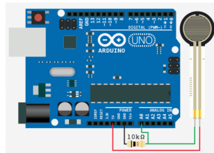
(b) Force-sensitive resistor .
