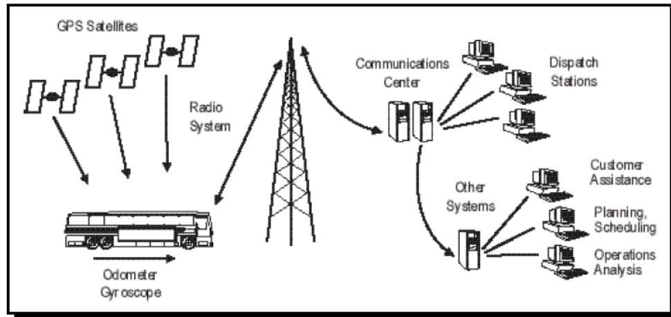
Figura 3.12. Funcionamiento GPS Fuente: (Transit Cooperative Research Program, 2008)
