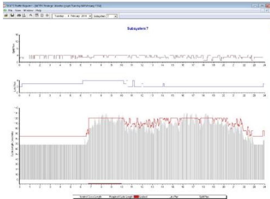
Figura 3.25. SCATS Traffic Reporter Fuente: (McCann, 2014)
