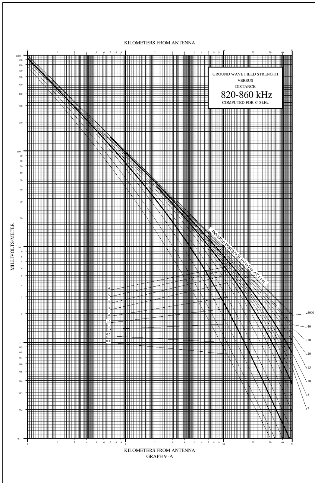
Figura E.3: Groud Wave Field Strength versus Distance 840[kHz] up to 50[km]
