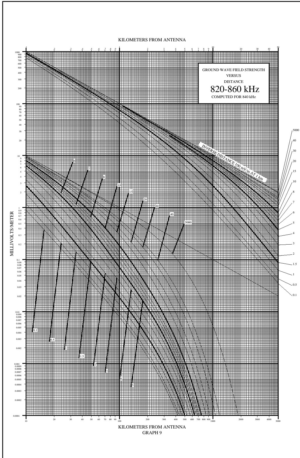
Figura E.2: Groud Wave Field Strength versus Distance 840[kHz]
