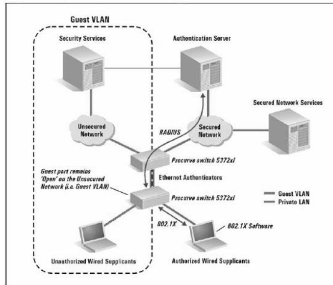
Figura 4.12 Arquitectura HP: Procurve Guest Access e Intelligent Management Center [49]
