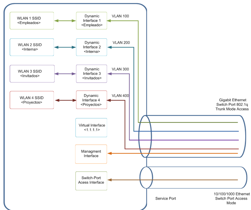
Figura 5.15 Interfaces WLC
