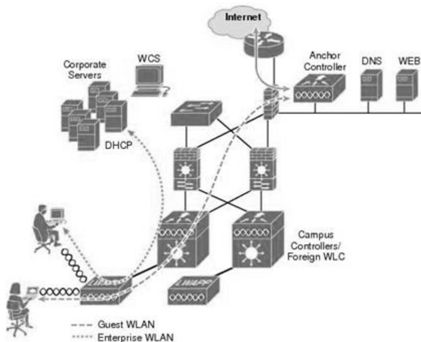
Figura 4.10 Arquitectura Cisco: Unified Wireless Guest Access Solution [47]
