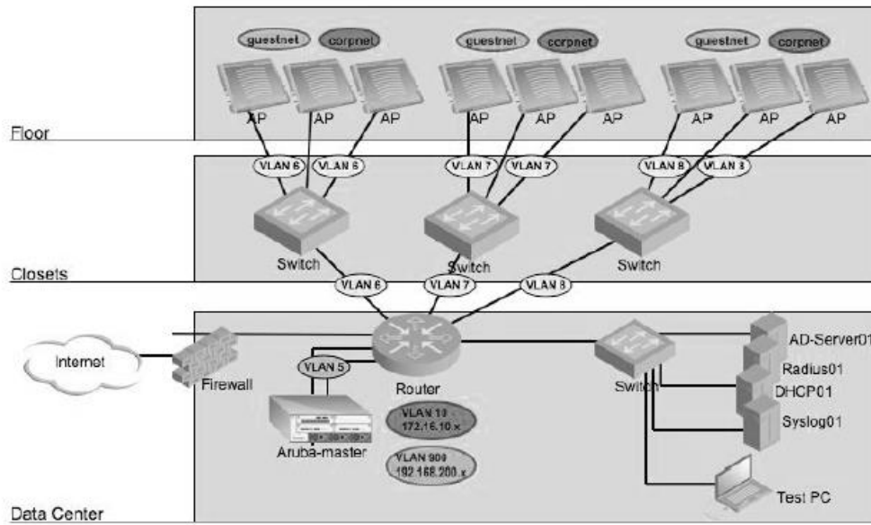
Figura 4.11 Arquitectura Aruba: Guest Access Solution [48]
