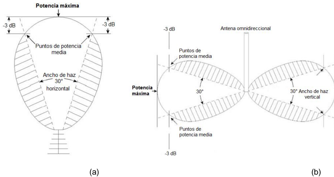
Figura 3.3 Ancho de haz: (a) horizontal; (b) vertical
