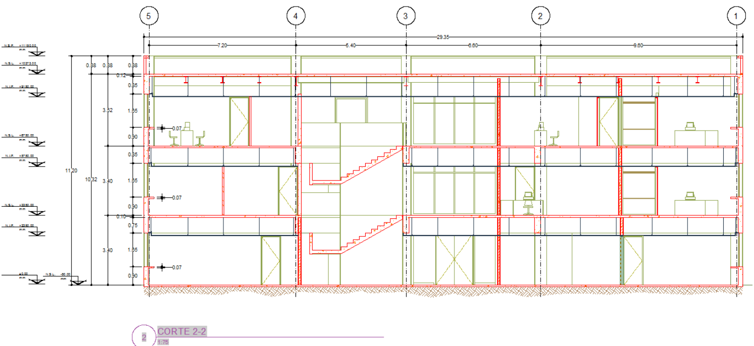
Figura 4-47 Corte transversal 2-2
