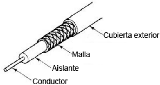
Figura 2.3. Cable coaxial.
