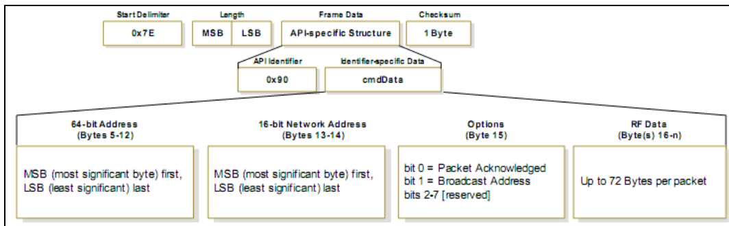
Figura 4.23 Zigbee Receive Packet
