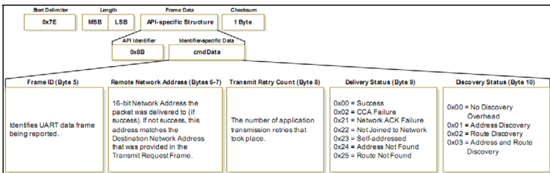
Figura 4.22 Zigbee Transmit Status
