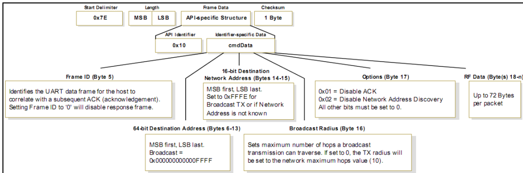
Figura 4.21 Trama Zigbee Transmit Request
