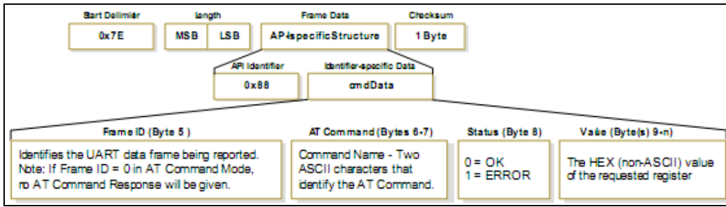
Figura 4.20 Trama AT Command Response
