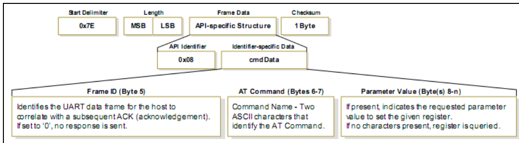
Figura 4.18 Trama AT Command
