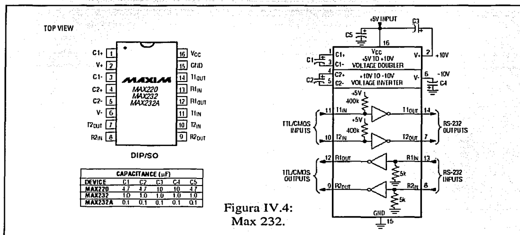
MAX220/MAX232/MAX232A Pin Configuration and Typical Operating Circuit
