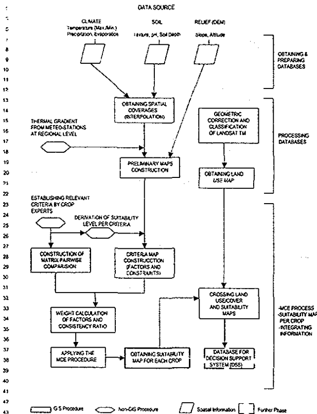
Fig. 2. This flow chart shows the main procedures applied in the Multi-Criteria Evaluation (MCE) approach.
