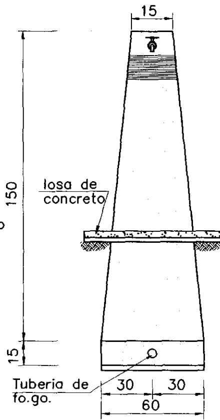
VISTA FRONTAL
