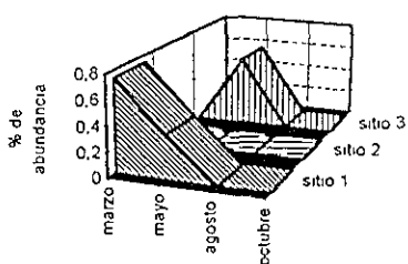
Gomphonema insignis
