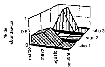
Gomphonema clavatum
