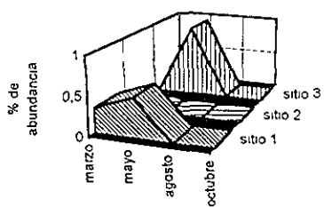
Gomphonema clavatum
