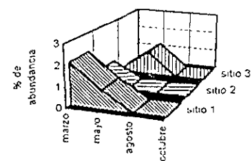
Gomphonema truncatum
