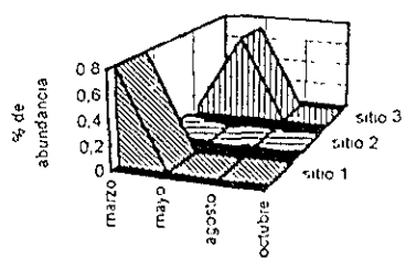
Gomphonema parvulum
