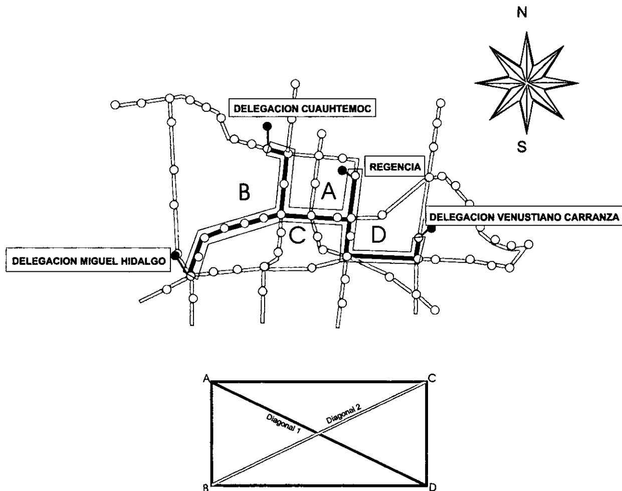
FIG.36. Backbone.
