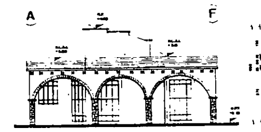
FACHADA PRINCIPAL
