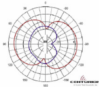
Elevation Plane Cut perpendicular to the antenna, parallel to the connector/cable exit, parallel to the polarization axis
