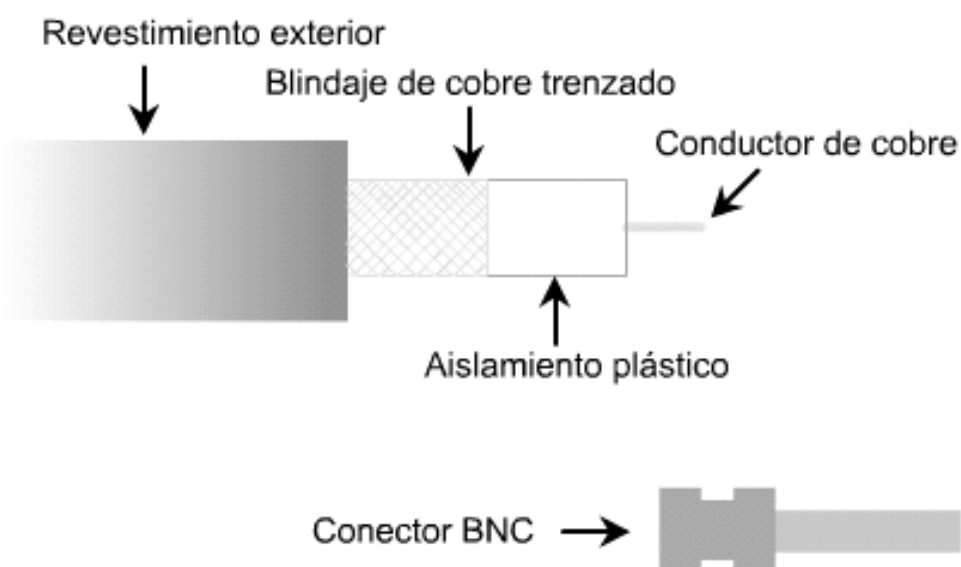
Figura IV.16. Cable coaxial.
