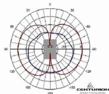
Omni Plane Cut in the plane of the antenna perpendicular to the connector/cable exit
