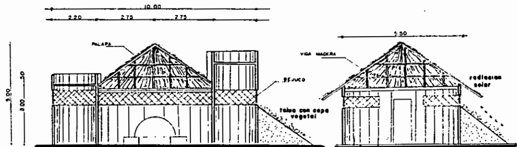
CORT X-X
